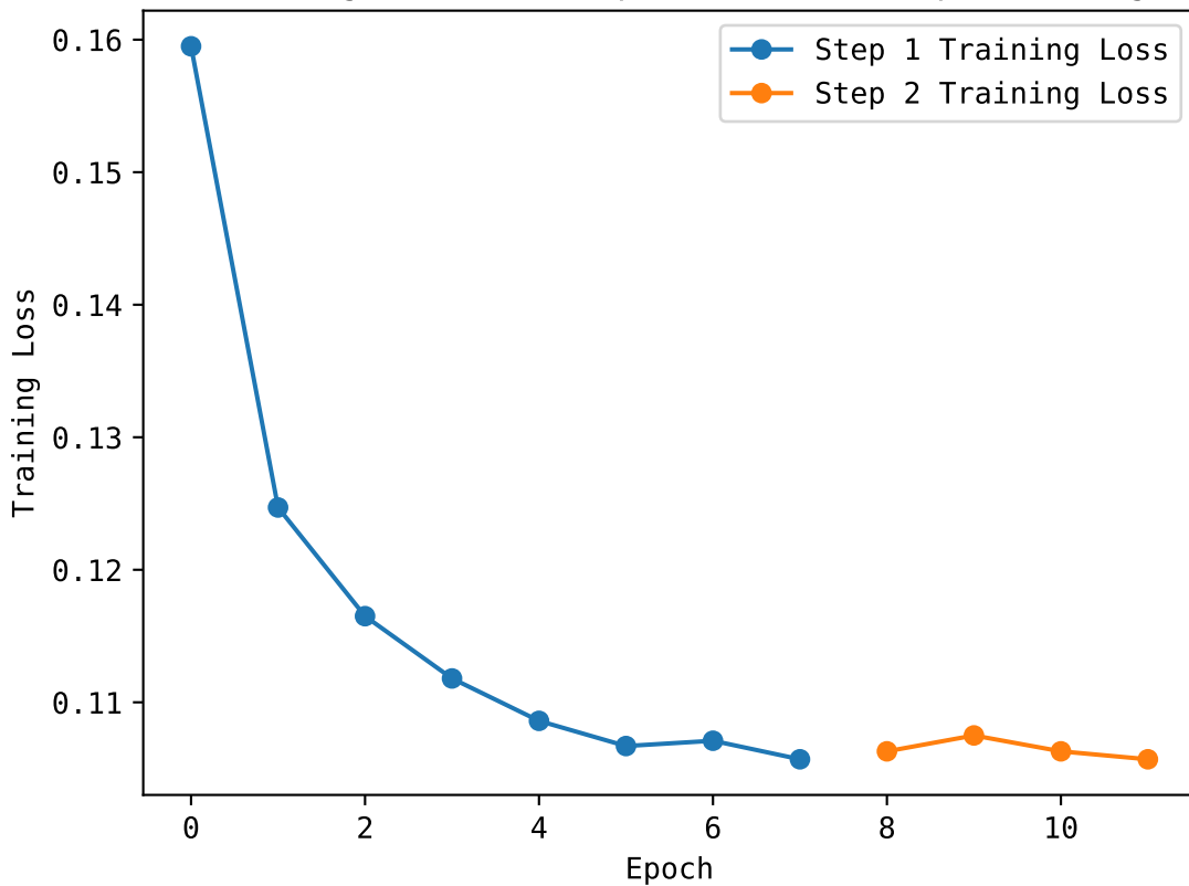
Training Loss over Epochs for 2-Step Training
