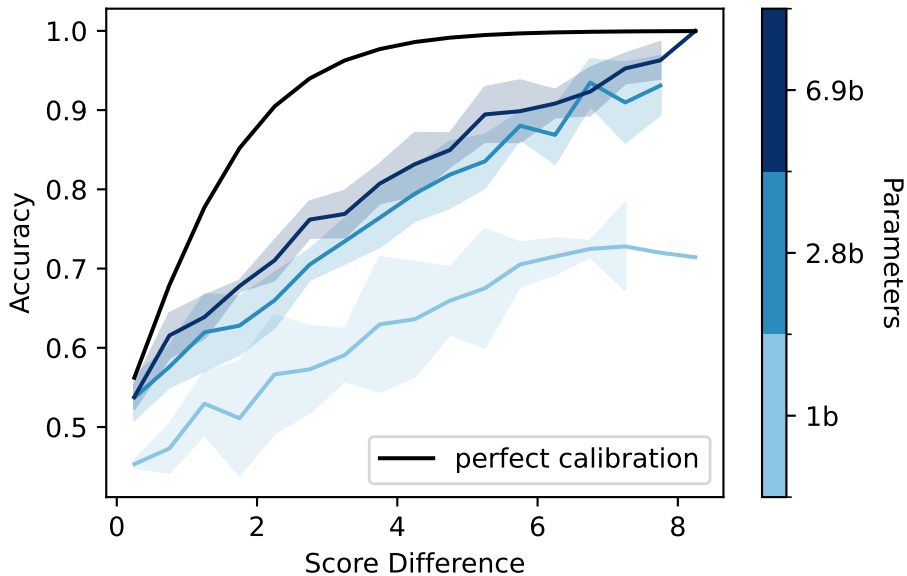
Calibration with GPT-3.5 turbo vs ground truth prediction
